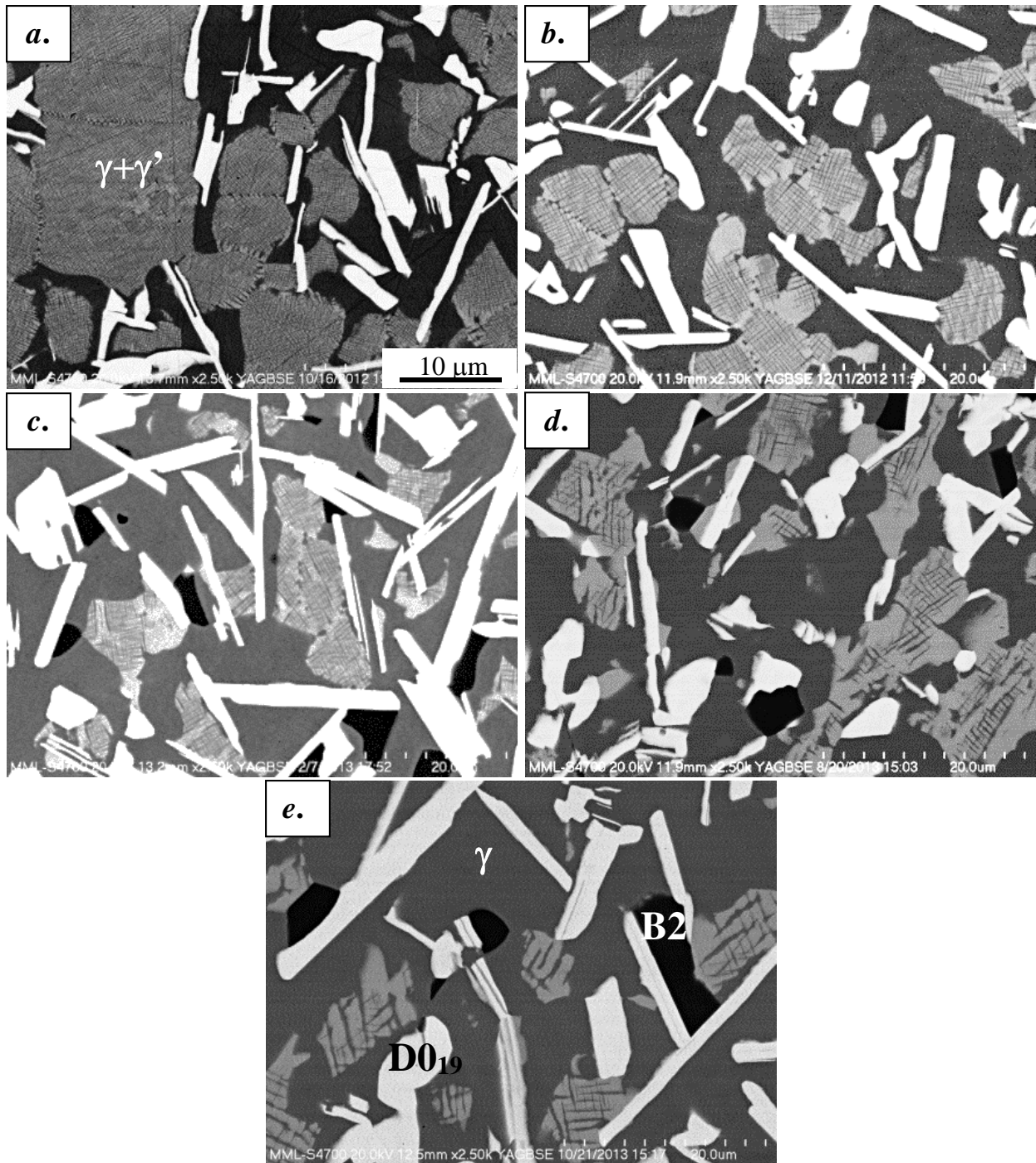
Figure 1: BSE micrographs of the L03 microstructure after annealing at 900 °C for a) 168 h, b) 1000 h, c) 2000 h, d) 4000 h, and e) 8000 h. The brightest phase in each image is D0 19 , black is B2, dark gray is γ and light gray is γ'. The scale bar in a) is representative of all images (i.e. the magnifications are the same).
